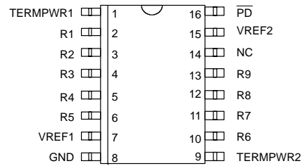
DS2107AS 16-Pin SOIC (300 mil)
